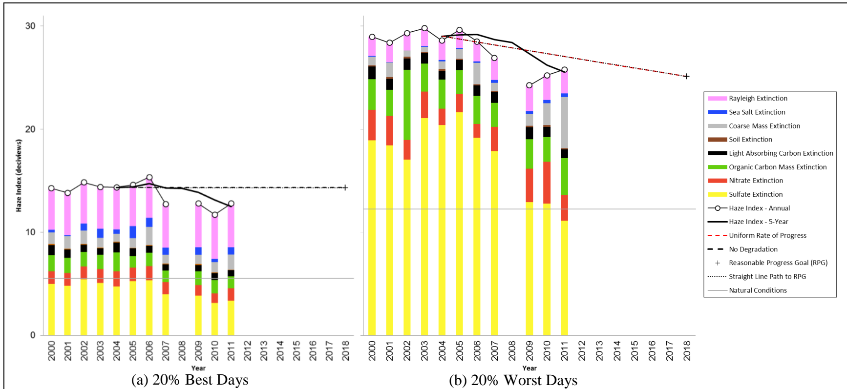
Figure 3-12. Individual Constituent Contribution to Annual Haze Index Levels at Brigantine Wilderness Area on 20 Percent Best and Worst Visibility Days
