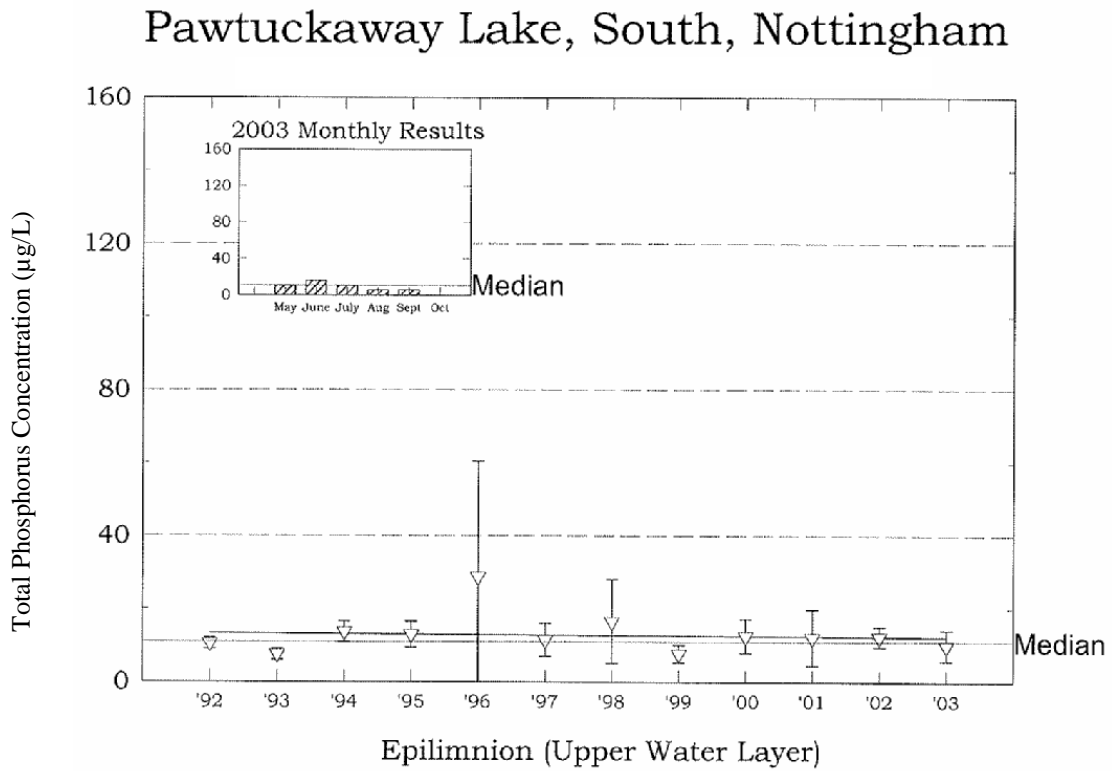
Figure 4: Historic Total Phosphorus Concentrations in the Epilimnion of Pawtuckaway Lake (Figure from NH-VLAP 2003 Biennial Report for Pawtuckaway Lake)
