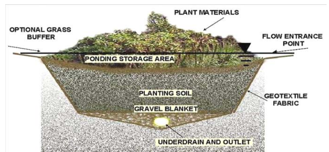
A cross-section of a typical bioretention cell.
