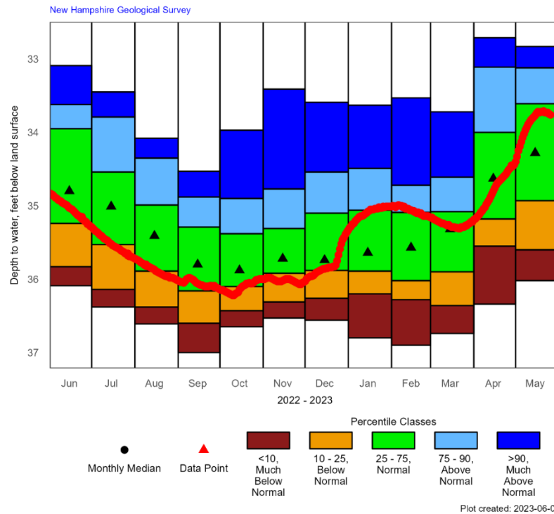
OXW-38: Ossipee, NH Overburden Well Annual Hydrograph with Historical Median and Percentile Classes
