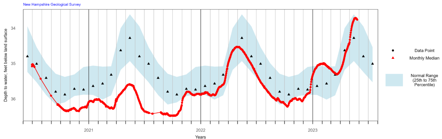
OXW-38: Ossipee, NH Overburden Well Groundwater Levels and Statistics for Past 3 Years
