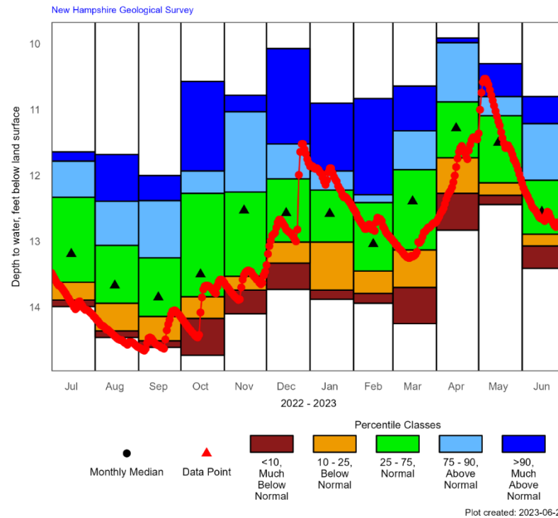
CBW-34: Campton, NH Overburden Well Annual Hydrograph with Historical Median and Percentile Classes
