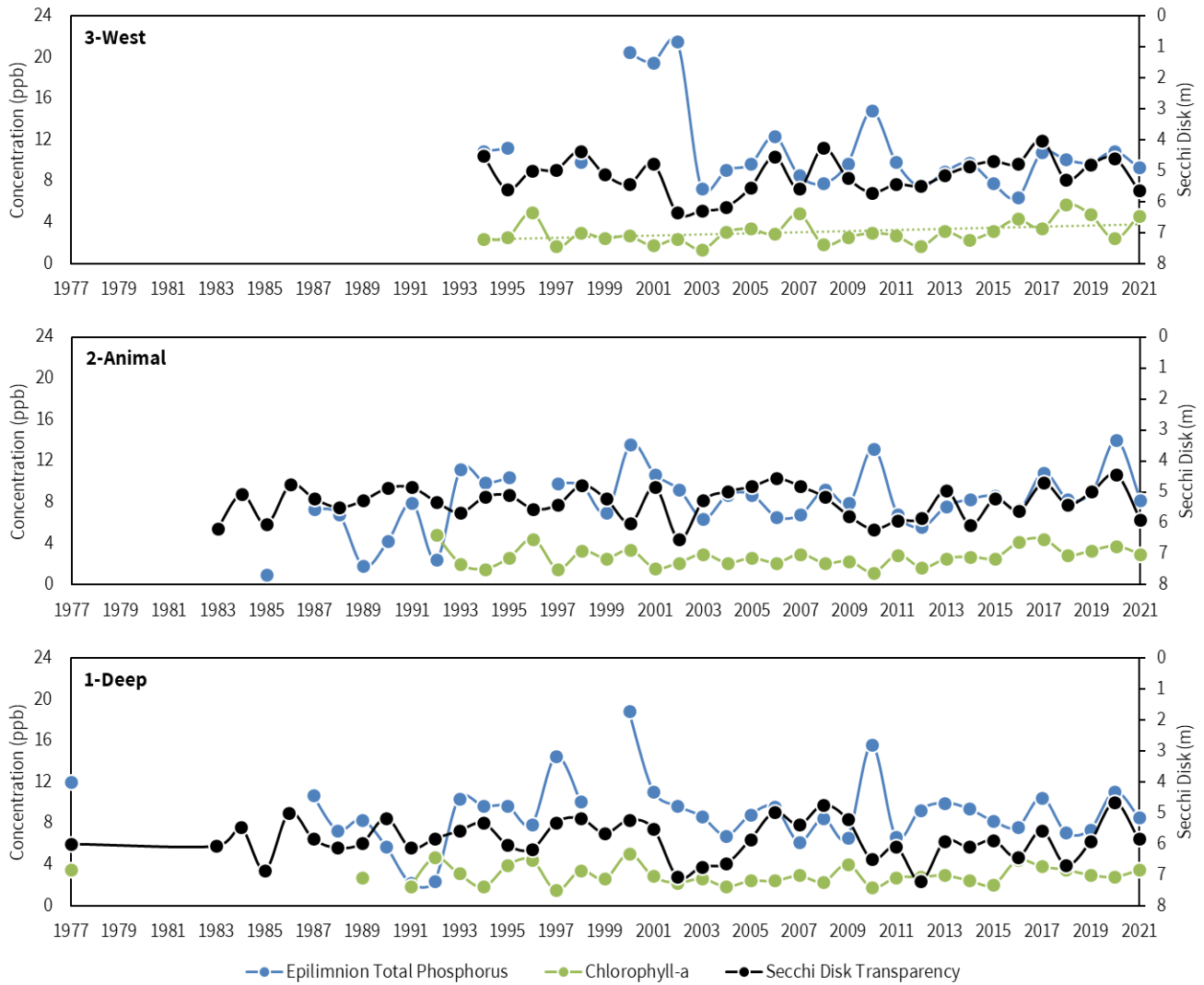
Figure 4. Median epilimnion total phosphorus, median epilimnion chlorophyll-a, and mean water clarity (Secchi Disk depth) measured at Lake Kanatka in June-September from 1977-2021 for stations 3-West (TOP), 2-Animal (MIDDLE), and 1-Deep (BOTTOM). Blooms were recorded in 2009, 2011, 2014, 2020, and 2021. A statistically significant increasing trend was detected for chlorophyll-a at 3-West ( p=0.0267 ) using rkt package in R.
