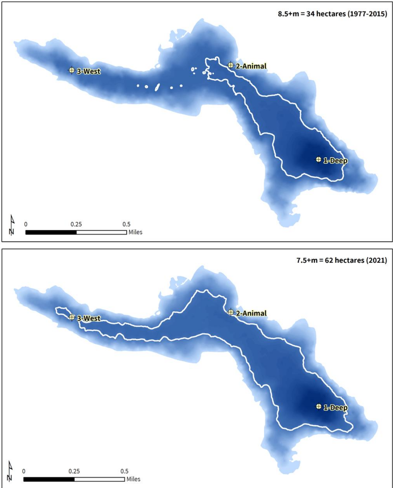
Figure 9. Bathymetric map depicting the increased extent of anoxia in Lake Kanasatka from 34 hectares at 8.5+ meters for dissolved oxygen profiles collected from 1977-2015 to 62 hectares at 7.5+ meters for dissolved oxygen profiles collected in 2021.
