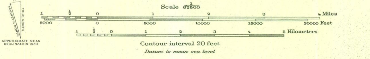
GEOLOGIC MAP AND STRUCTURE SECTIONS OF THE PERCY QUADRANGLE, NEW HAMPSHIRE
