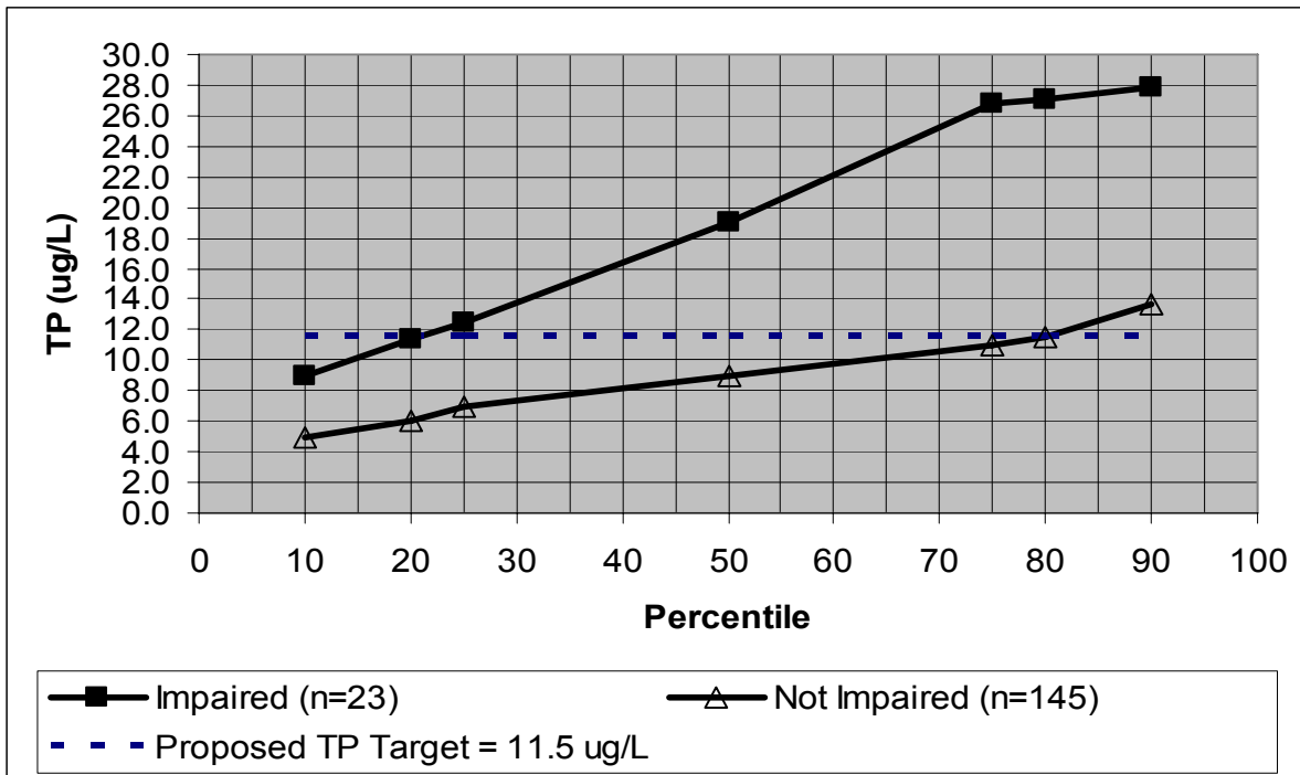
Figure A-2: Cumulative Frequency Distribution of TP Concentrations in Impaired and Unimpaired New Hampshire Lakes.
