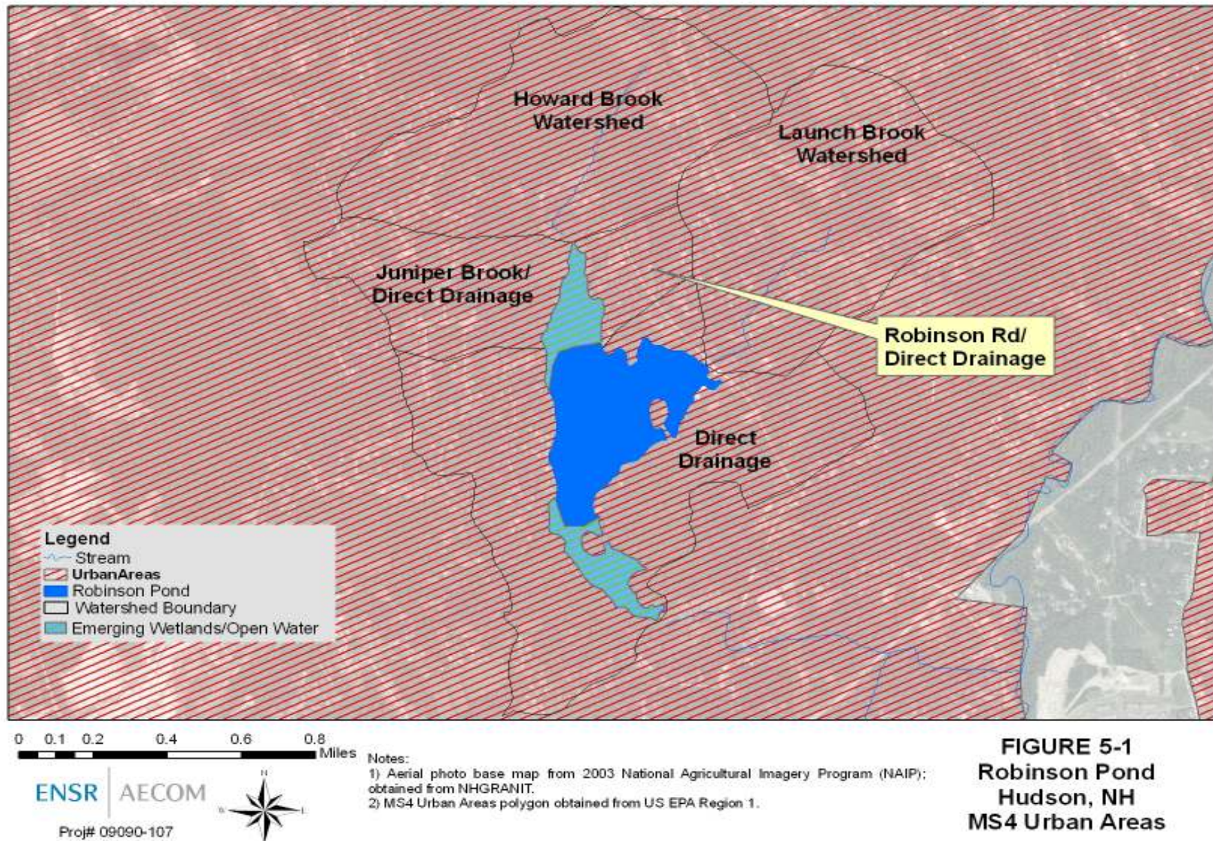
Figure 5-1. MS4 Urbanized Areas in Robinson Pond Watershed.
