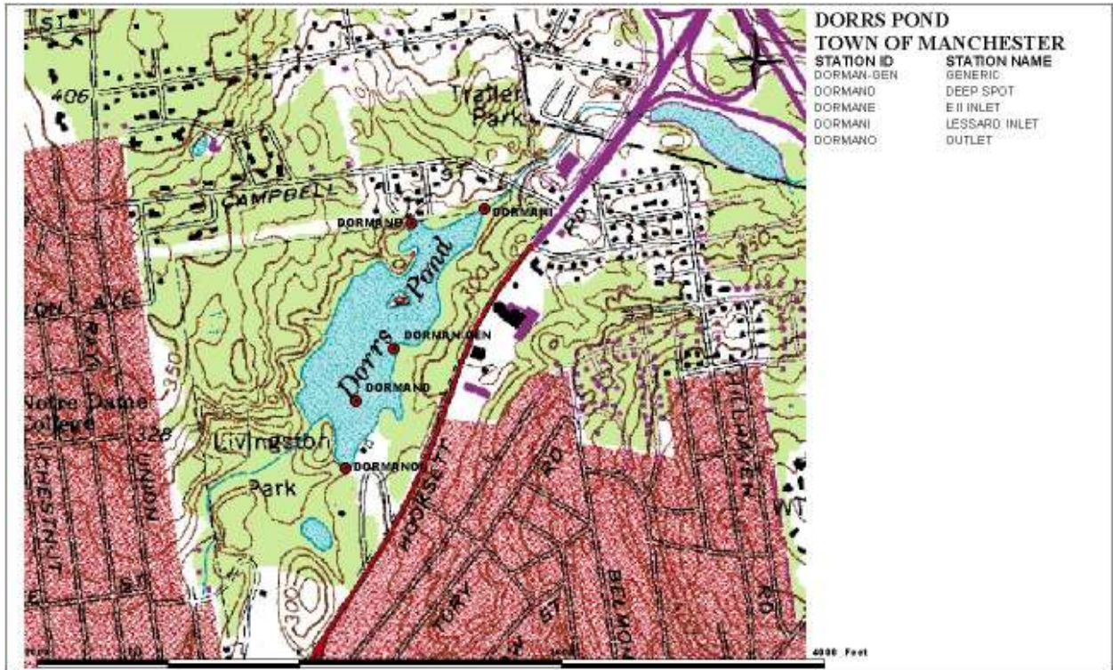
Figure 8-1. NH DES Sampling Locations in Dorrs Pond.
