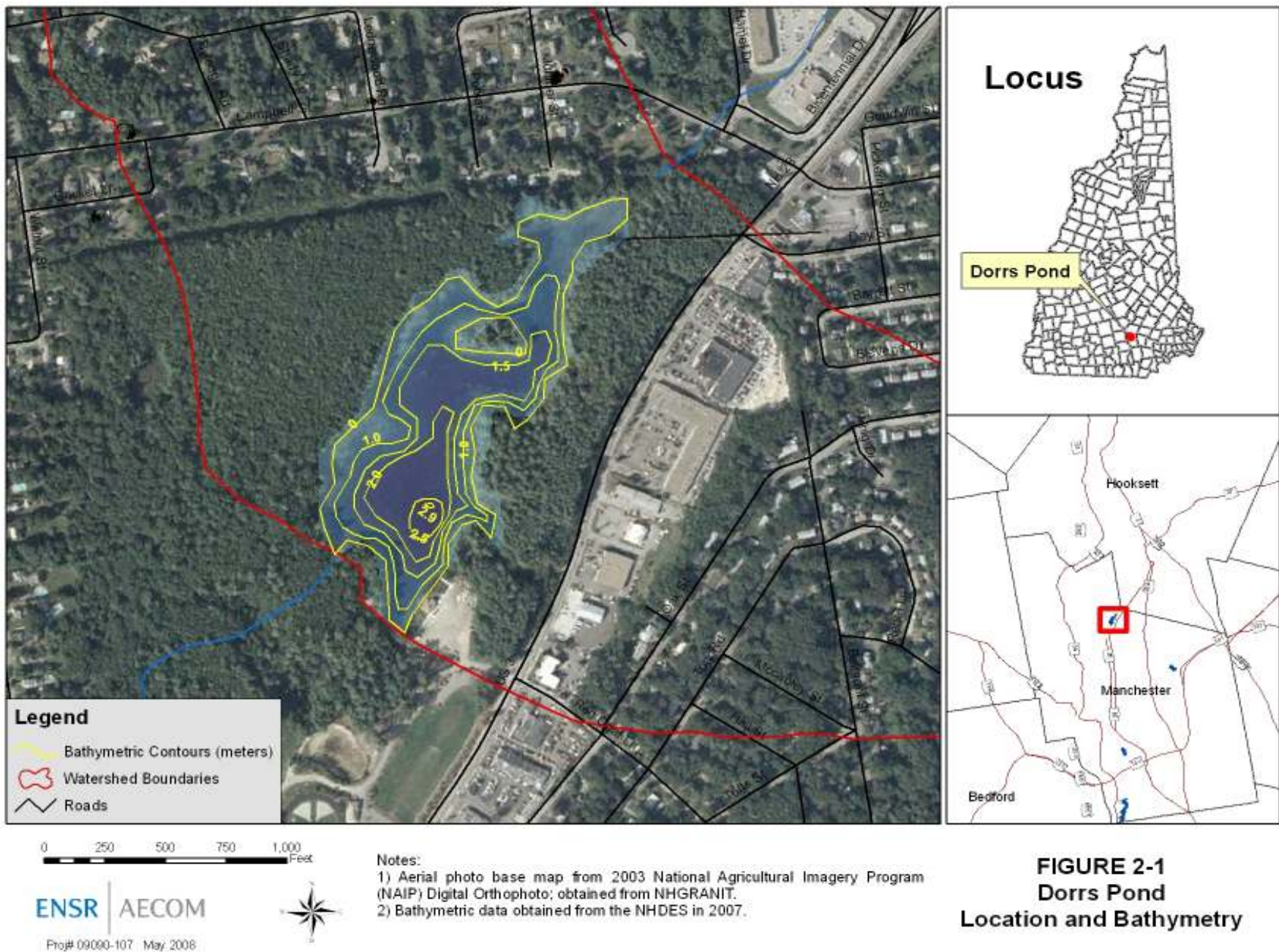
Figure 2-1. Dorrs Pond Location and Bathymetry.
