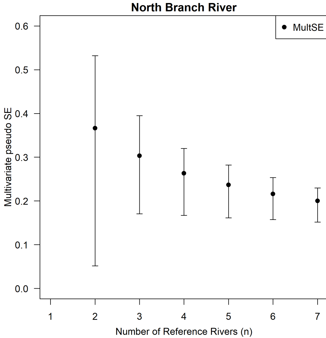
Figure - 8: MultSE for the final reference river selection.
