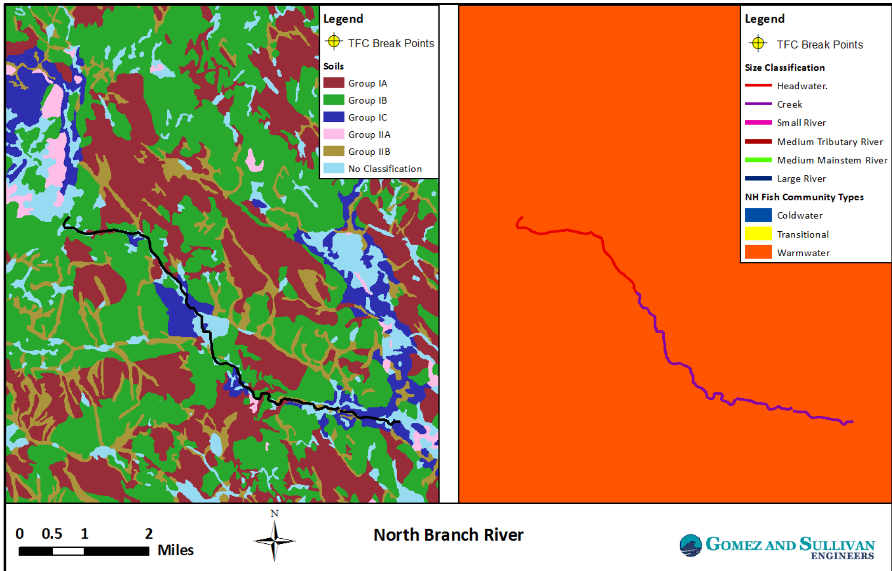
Figure - 2: Soils (left panel), watershed size-class (right panel), and NH predicted fish community types (right panel).
