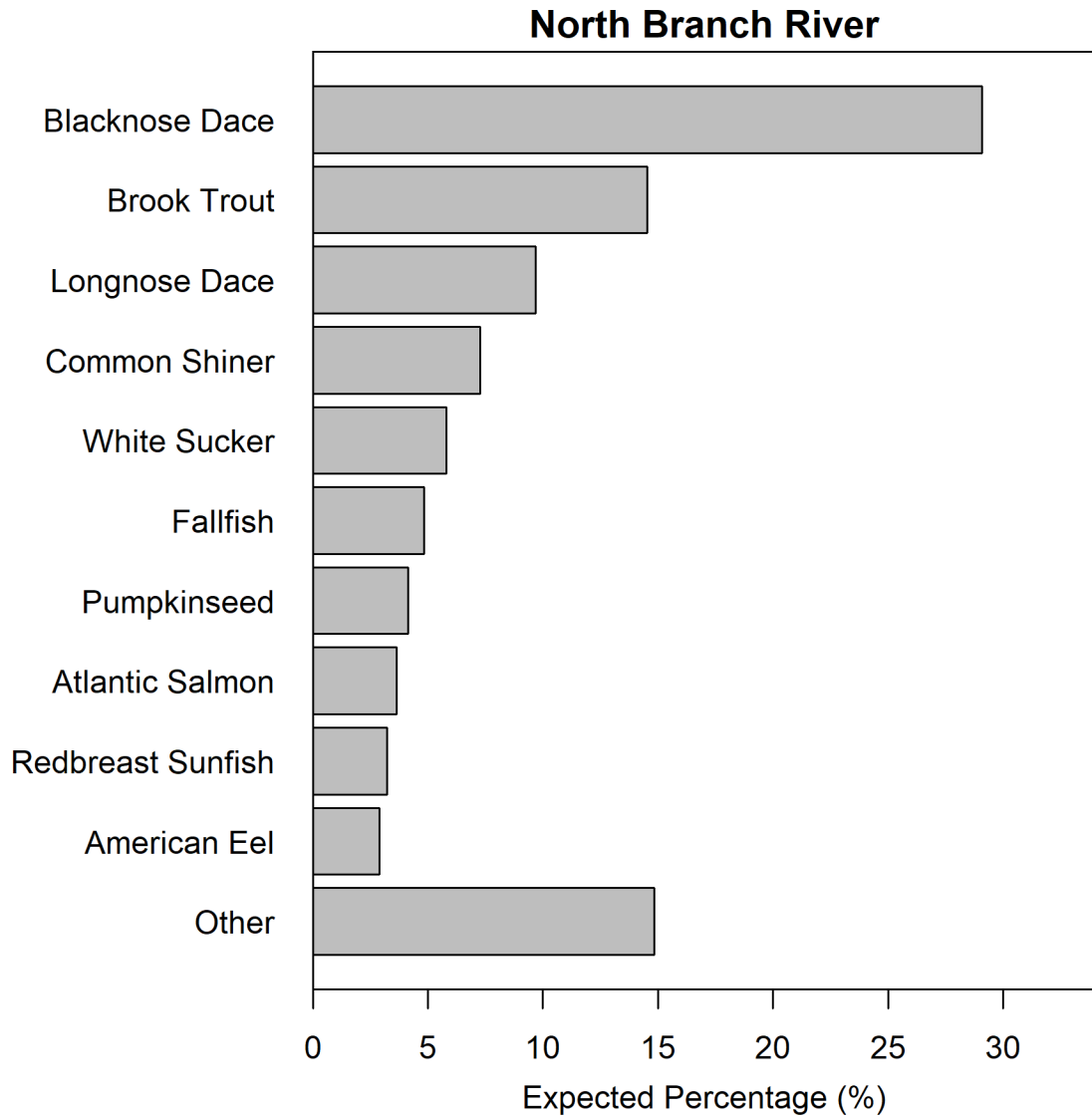
Figure - 10: Graphical representation of the TFC Model for the North Branch River.
