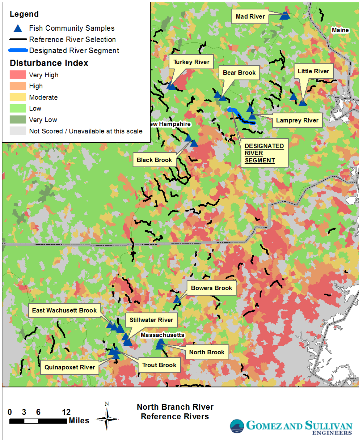
Figure - 6: Initial selection of reference river fish community samples.
