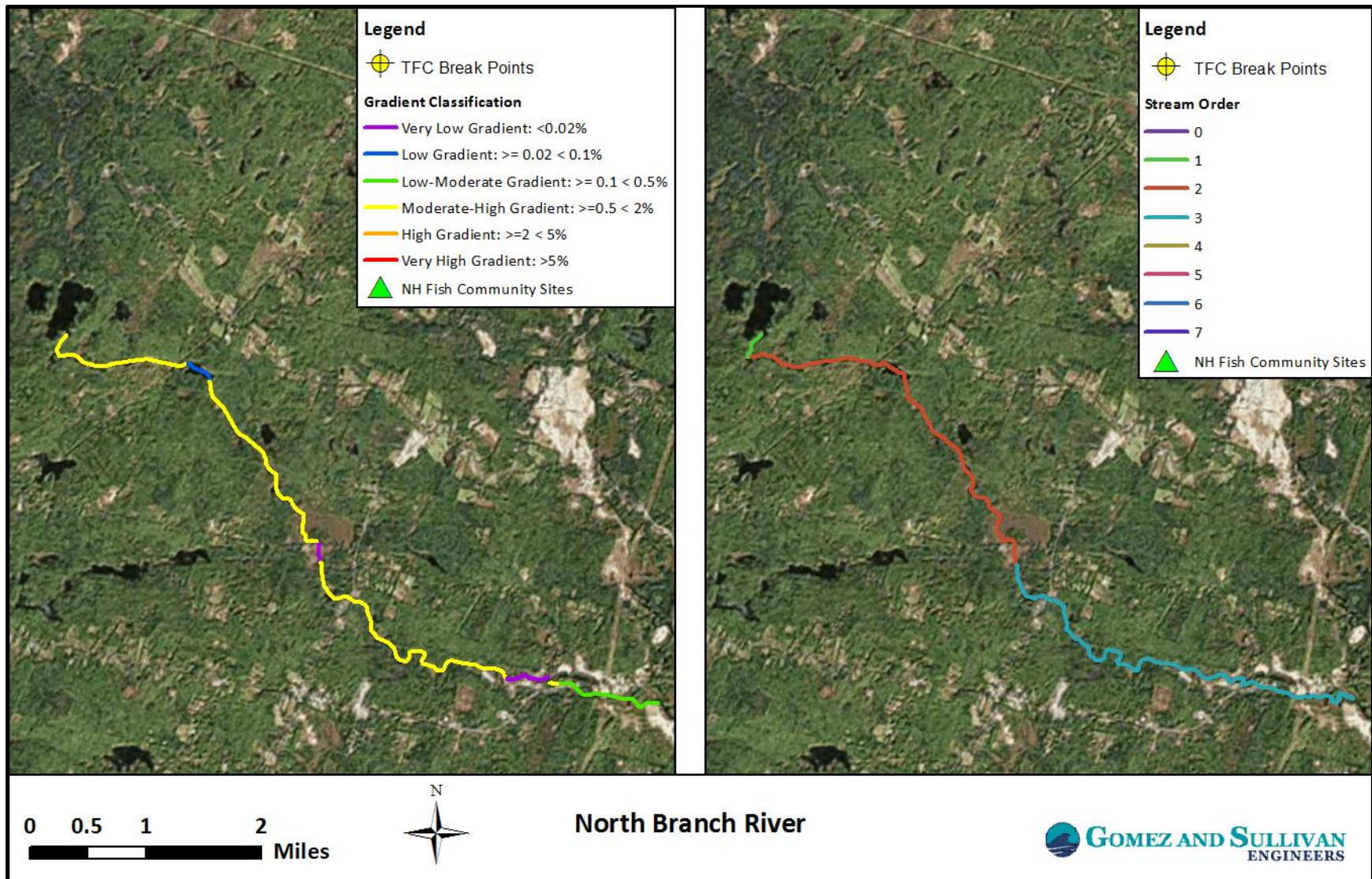
Figure - 1: Gradient (left panel) and stream order (right panel), along with fish sampling locations.
