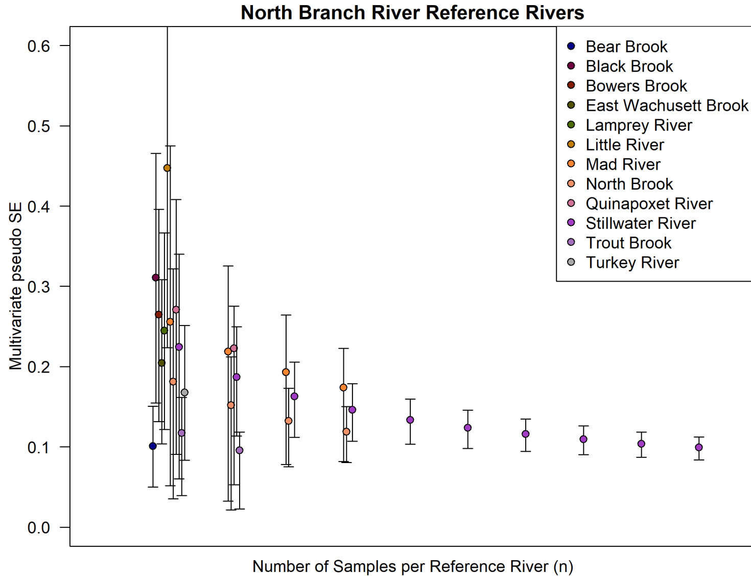
Figure - 7: MultSE (beginning at n=2) of fish community data for reference rivers initially selected.
