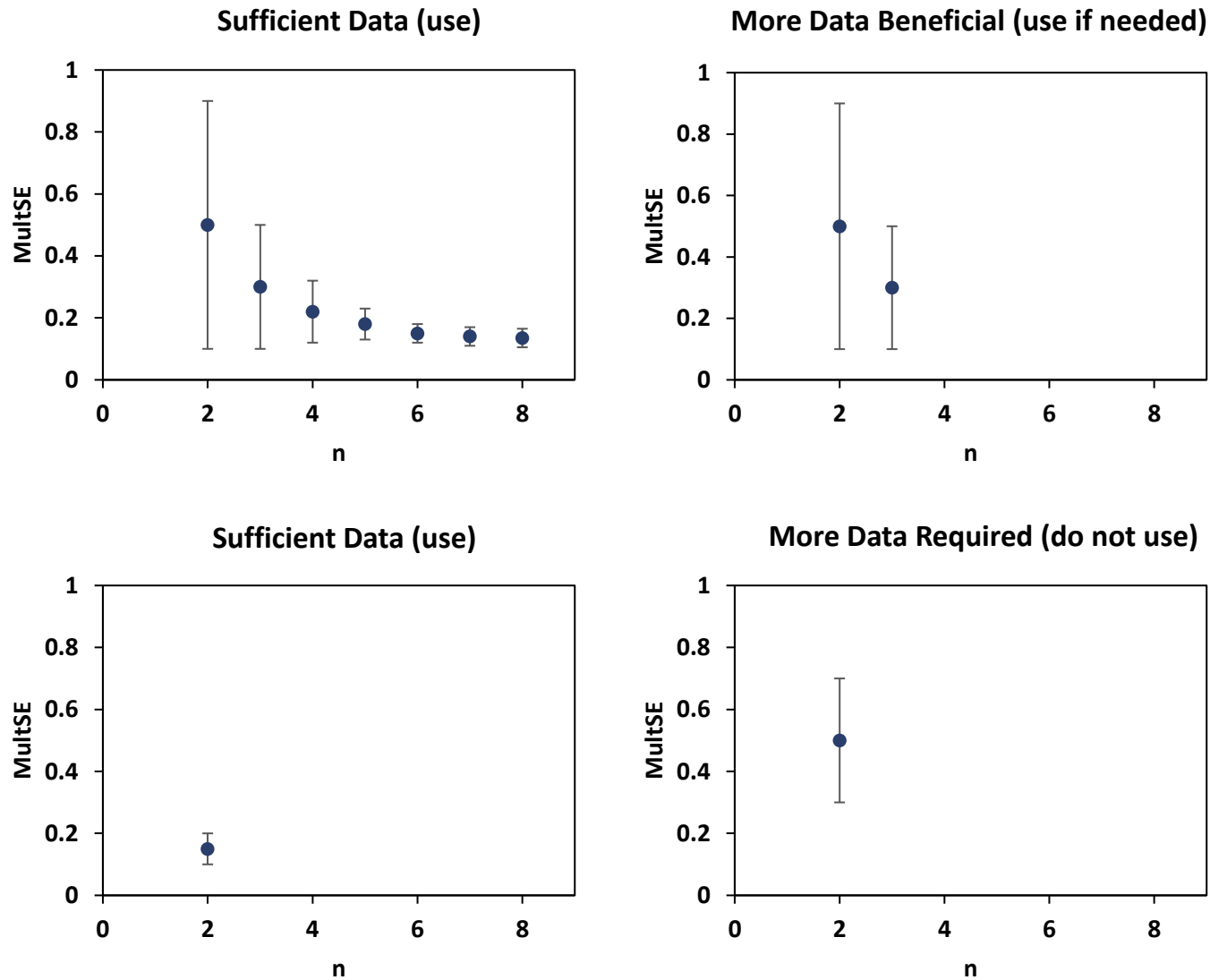
Figure - 5: Theoretical example of evaluating the number of samples (i.e. whether data are sufficient for further analysis) using MultSE.
