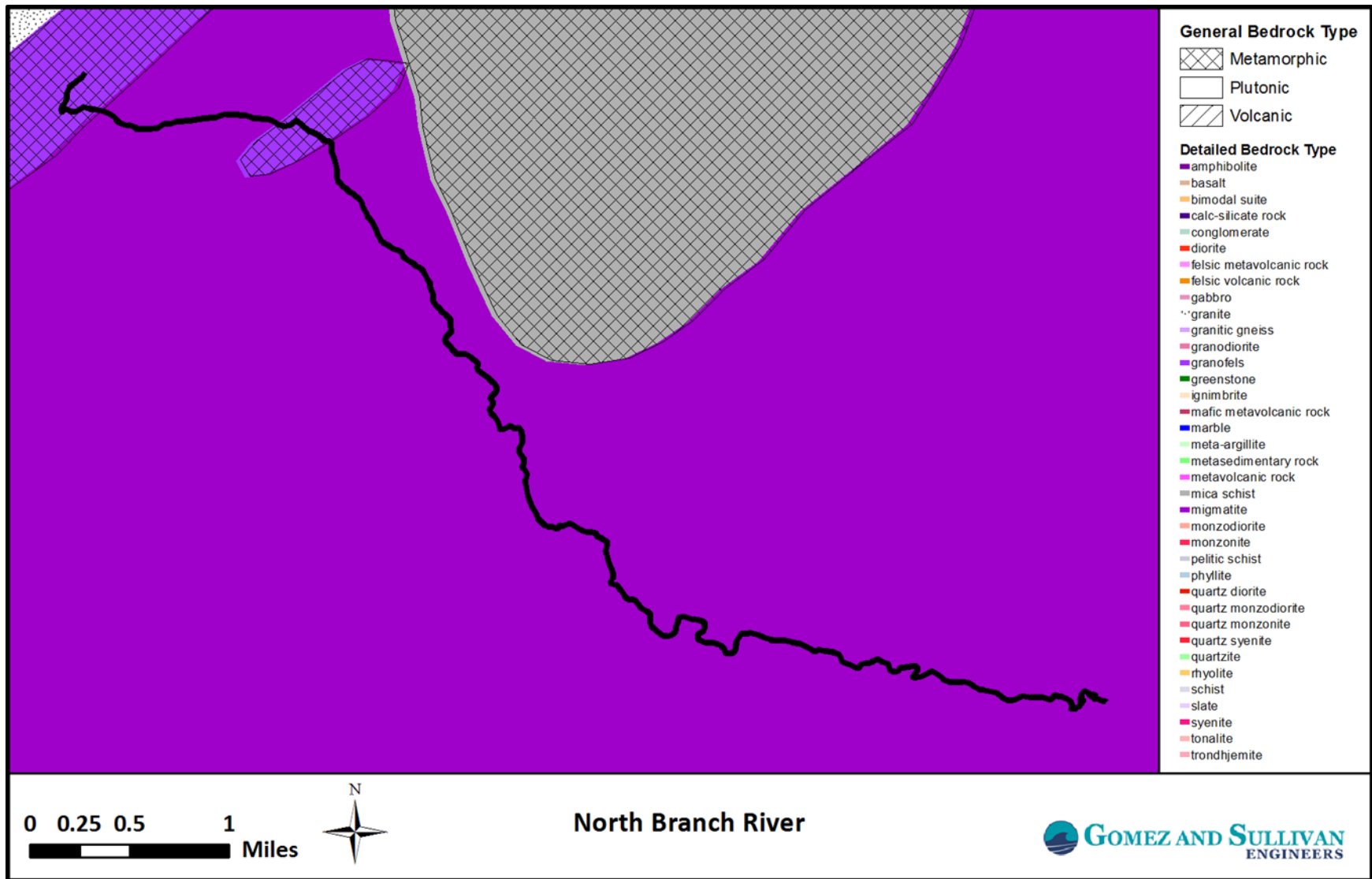
Figure - 3: Bedrock composition and water chemical classification.
