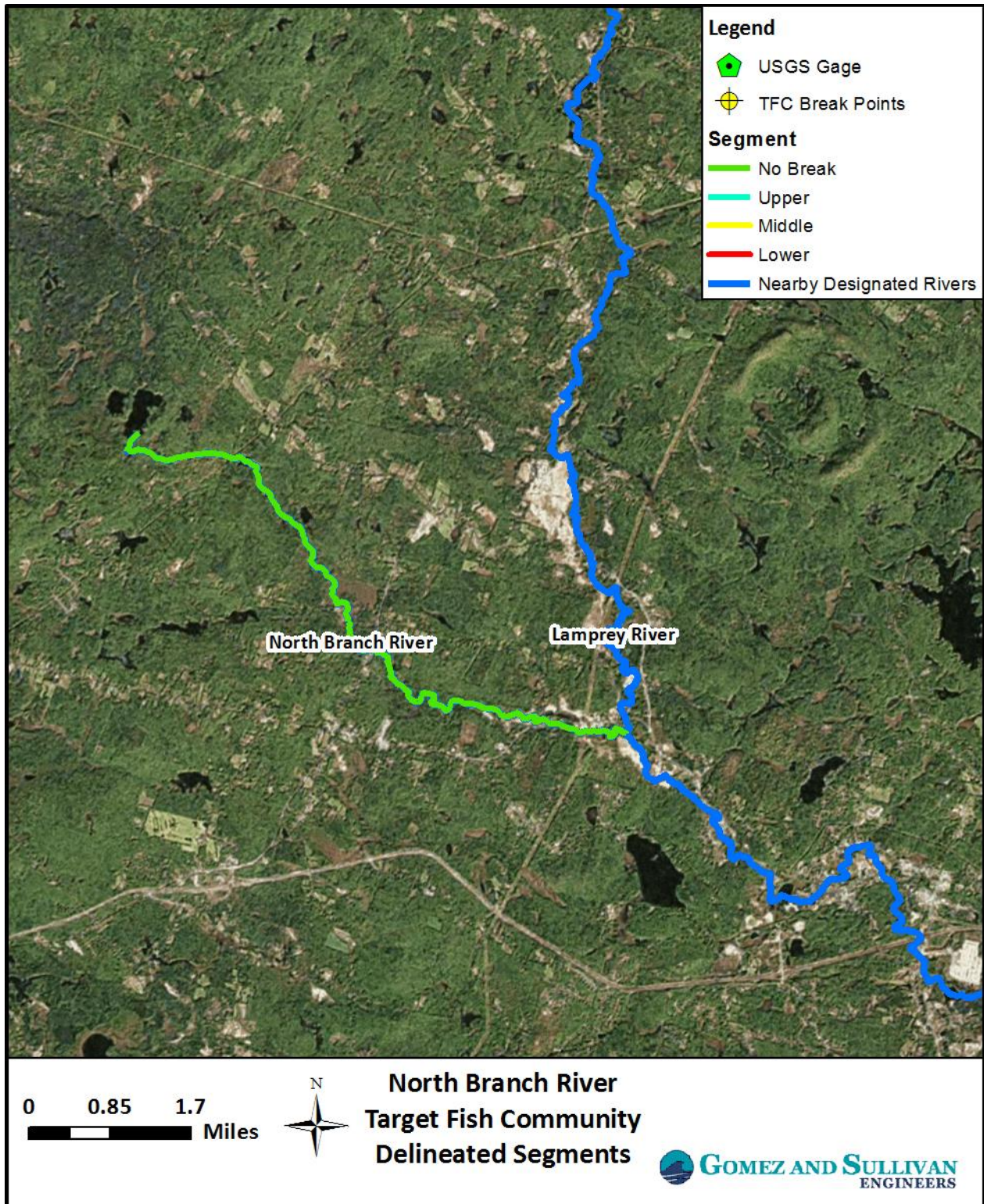
Figure - 4: Delineated segments derived from the TFC break points.
