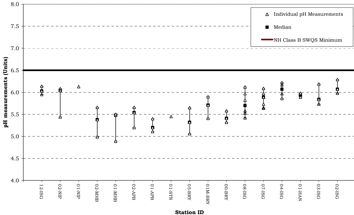
Figure 2. pH Statistics for the Isinglass River Watershed June 25 - October 9, 2009, NHDES VRAP
