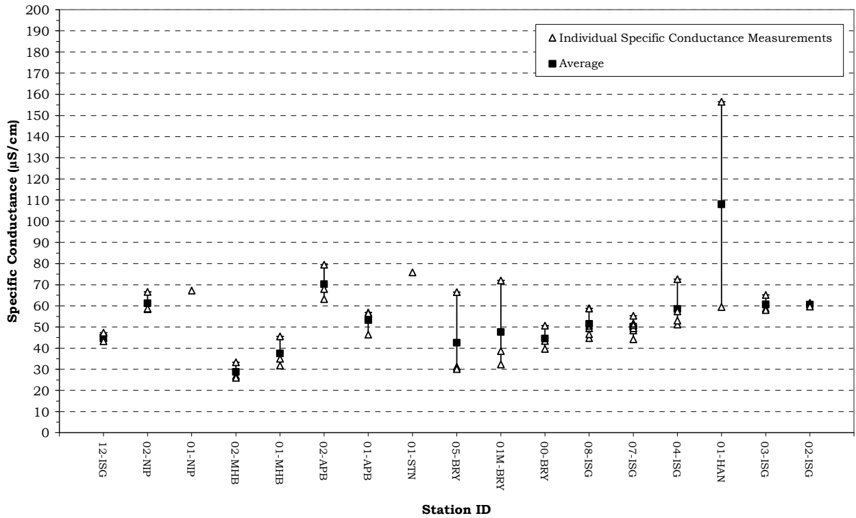
Figure 4. Specific Conductance Statistics for the Isinglass River June 25 - October 9, 2009, NHDES VRAP
