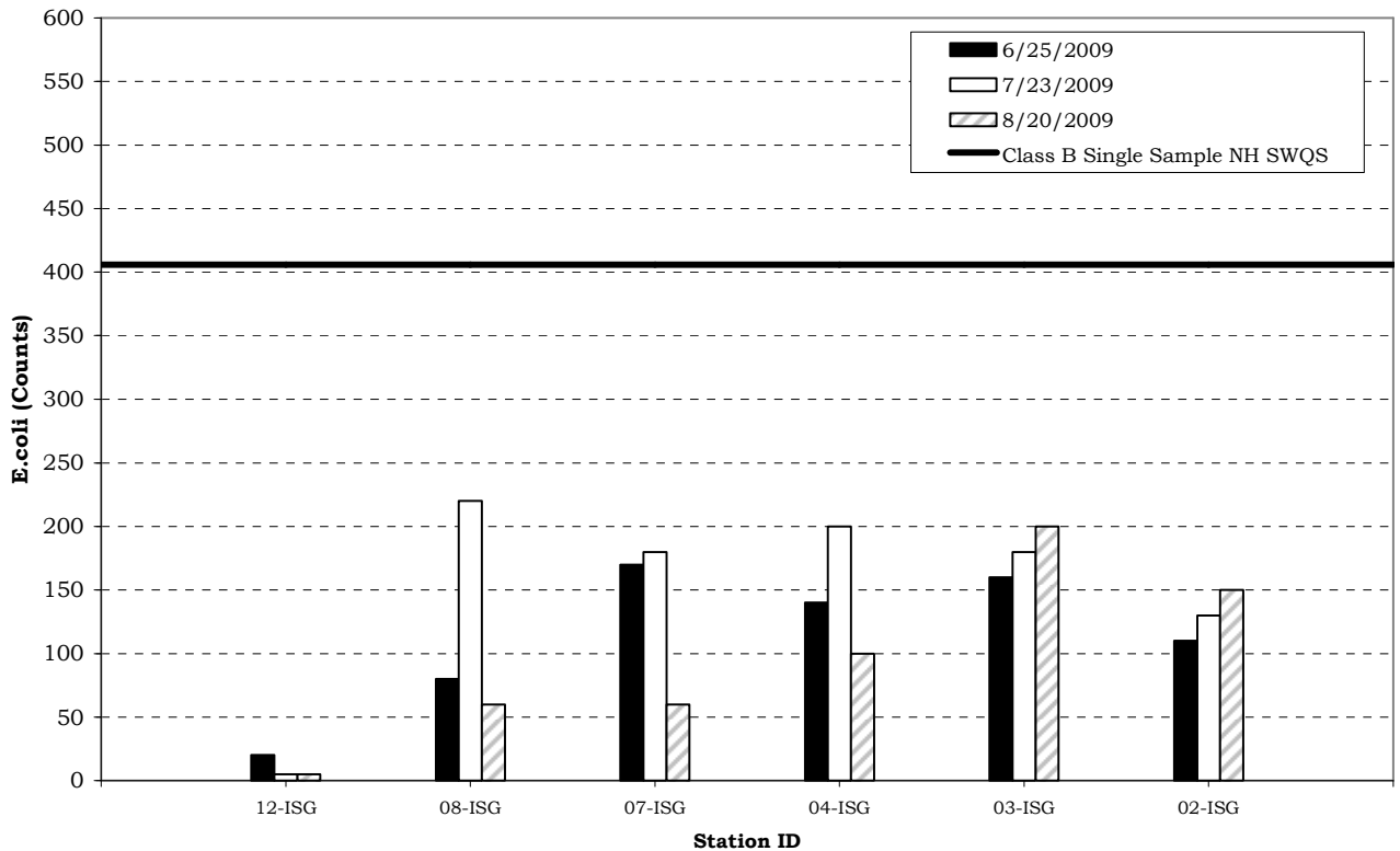
Figure 6. Escherichia coli Statistics for the Isinglass River Watershed June 25 - August 20, 2009, NHDES VRAP
