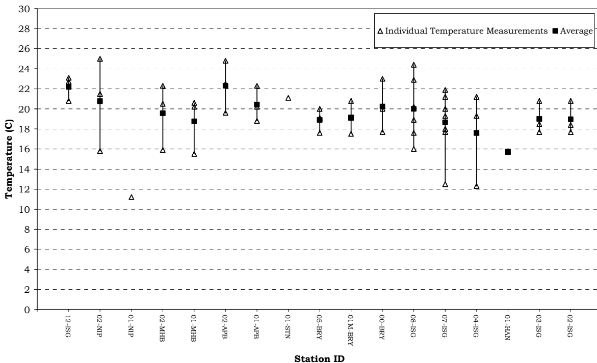
Figure 5. Water Temperature Statistics for the Isinglass River June 25 - October 9, 2009, NHDES VRAP
