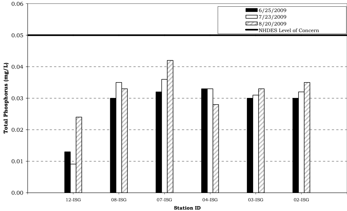
Figure 7. Total Phosphorus Statistics for the Isinglass River Watershed June 25 - August 20, 2009, NHDES VRAP
