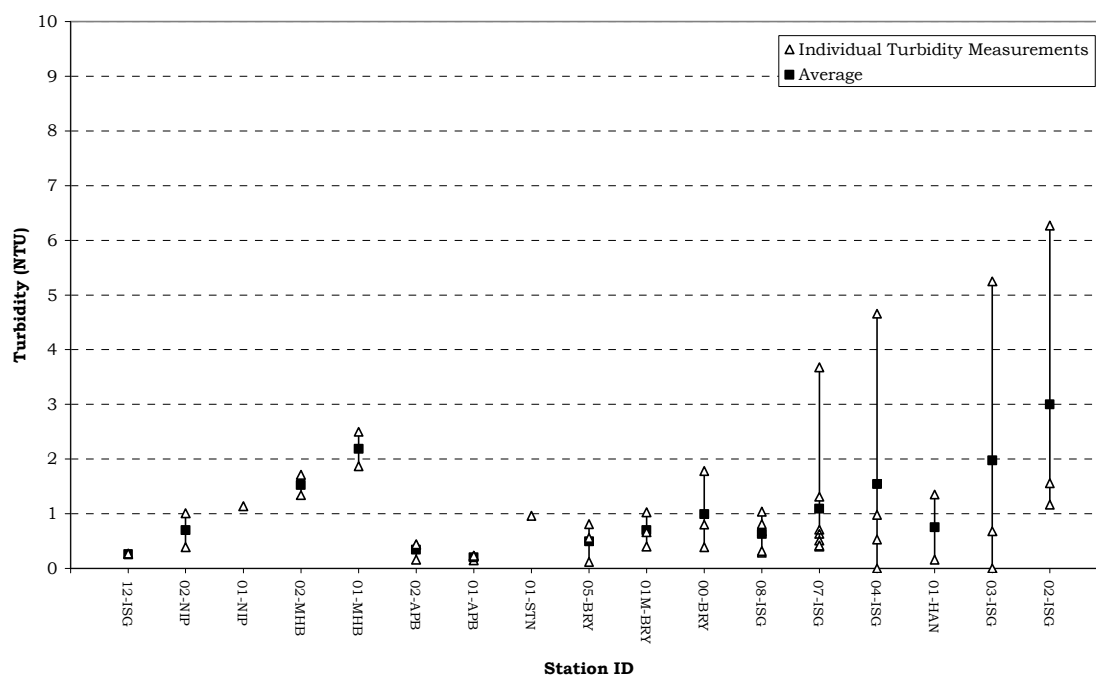
Figure 3. Turbidity Statistics for the Isinglass River Watershed June 25 - October 9, 2009, NHDES VRAP
