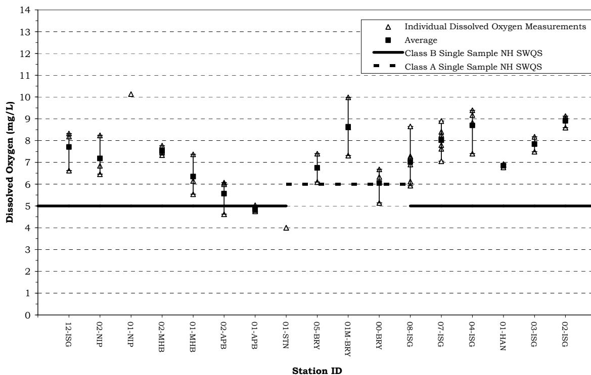
Figure 1. Dissolved Oxygen Concentration Statistics for the Isinglass River Watershed June 25 - October 9, 2009, NHDES VRAP
